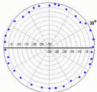
Elevation Coordinate Pattern Plot – WIFI-PLUS MP- BULLET Antenna
