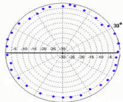
Elevation Coordinate Pattern Plot -- WIFI-PLUS MP- BULLET Antenna
