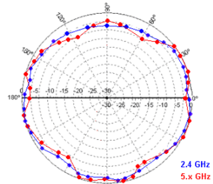
Elevation Coordinate Pattern Plot UWB-BULLET antenna by WIFI-PLUS
